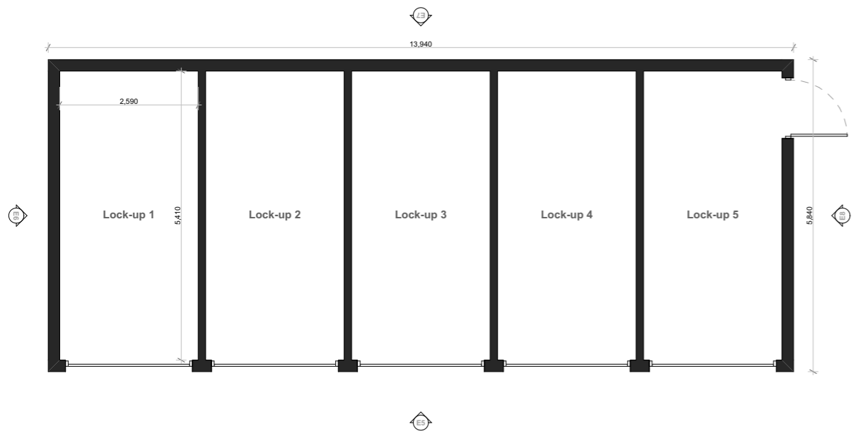
1:100 Floor Plan
