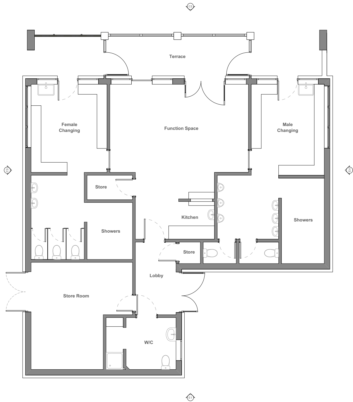
1:100 Existing Ground Floor
